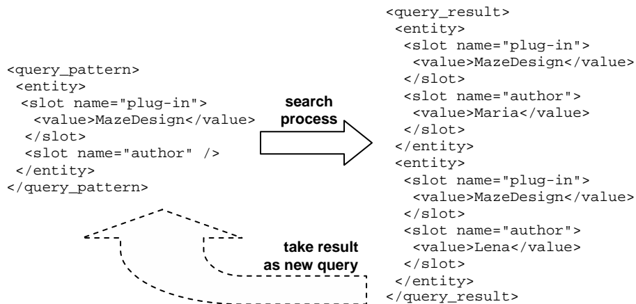
Fig. 2. XML representations of retrieval queries and answers
